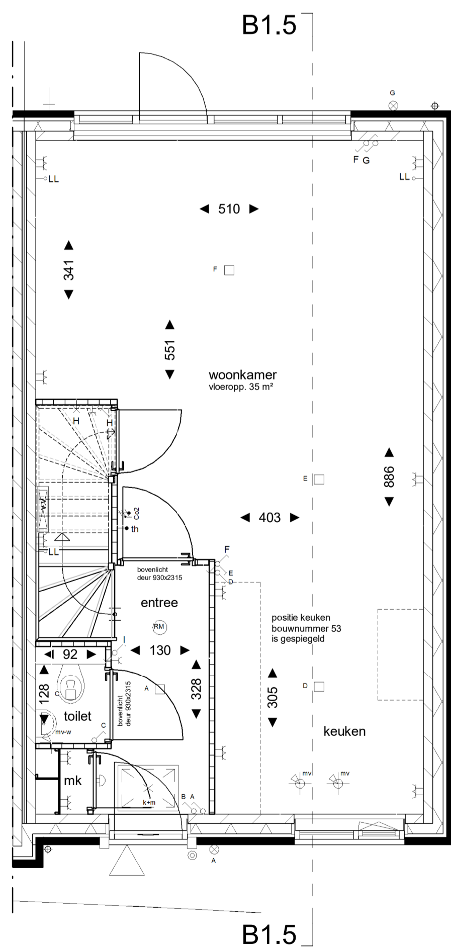
bnr: 22, 46 en 51 type C1sp Begane grond 1:50
